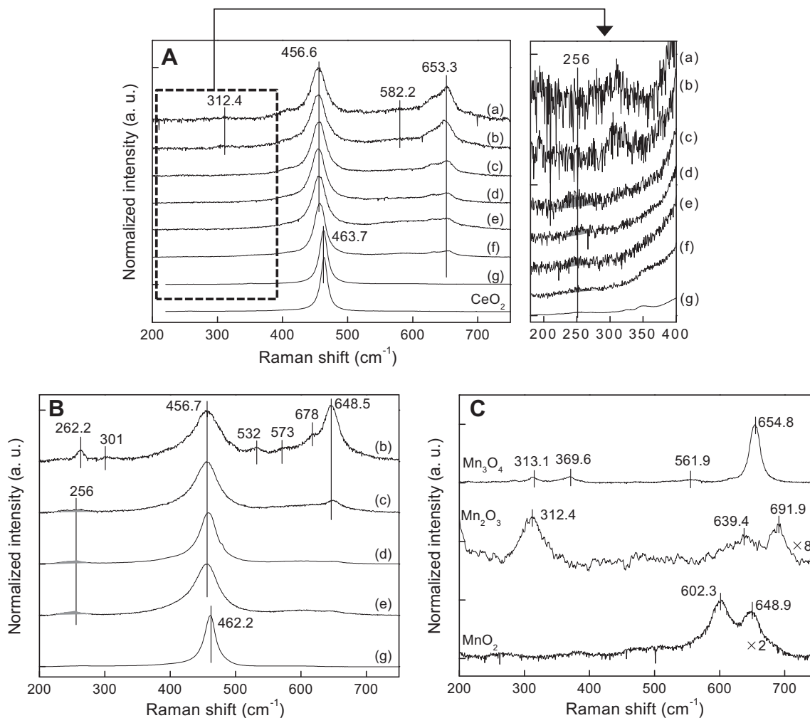
Fig. 8. Raman spectra of the BaO/Ce-Mn( x ) catalysts (A), Ce-Mn( x ) calcined at 400 °C (B), and Mn references (C): (a) x = 0.8; (b) x = 0.75; (c) x = 0.5; (d) x = 0.25; (e) x = 0.2; (f) x = 0.1; and (g) x = 0. Raman spectrum of a single-component CeO 2 without Ba (Ce-Mn(0)) calcined at 800 °C is also given in A. The Raman peak at 256 cm -1 due to the defect structure of CeO 2 is indicated by shade.
