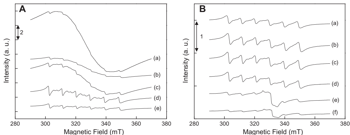
Fig. 4. ESR spectra of Ce-Mn( x ) calcined at 400 °C (A) and BaO/Ce-Mn( x ) catalysts (B): (a) x = 0.8 ; (b) x = 0.75 ; (c) x = 0.5 ; (d) x = 0.25 ; (e) x = 0.2 ; and (f) x = 0.1 .
