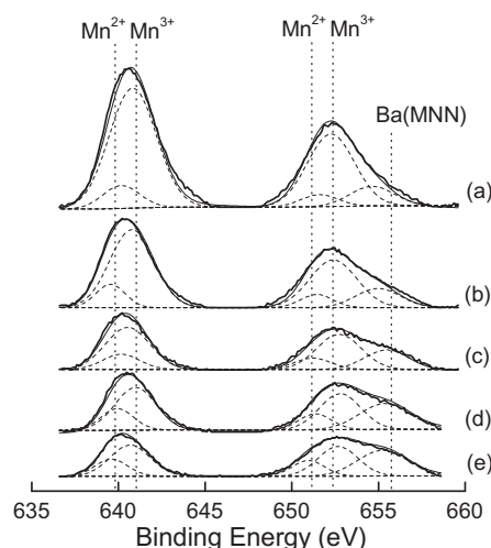
Fig. 6. Mn 2p XPS spectra of the BaO/Ce–Mn( x ) catalysts: (a) x = 0.75; (b) x = 0.5; (c) x = 0.25; (d) x = 0.2; and (e) x = 0.1.
