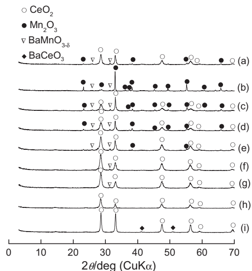
Fig. 3. XRD patterns of BaO/Ce–Mn( x ) catalysts calcined at 800 °C for 1 h: (a) BaO (physical mixture of CeO 2 and Mn 2 O 3 ), (Ce/(Ce+Mn) = 0.5); (b) BaO/Ce–Mn(1.0); (c) BaO/Ce–Mn(0.8); (d) BaO/Ce–Mn(0.75); (e) BaO/Ce–Mn(0.5); (f) BaO/Ce–Mn(0.25); (g) BaO/Ce–Mn(0.2); (h) BaO/Ce–Mn(0.1); and (i) BaO/Ce–Mn(0).
