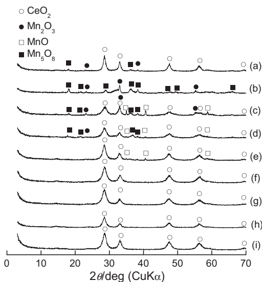
Fig. 2. XRD patterns of Ce–Mn( x ) calcined at 400 °C for 4 h: (a) physical mixture of Ce–Mn(0) and Ce–Mn(1.0) (Ce/(Ce + Mn) = 0.5, mixed after calcination at 400 °C); (b) Ce–Mn(1.0); (c) Ce–Mn(0.8); (d) Ce–Mn(0.75); (e) Ce–Mn(0.5); (f) Ce–Mn(0.25); (g) Ce–Mn(0.2); (h) Ce–Mn(0.1); and (i) Ce–Mn(0).
