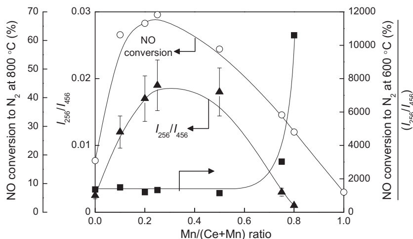
Fig. 9. Effect of the Mn/(Ce+Mn) ratio on I_{256}/I_{456} calculated from the Raman spectrum of the BaO/Ce–Mn( x ) catalyst. For comparison, NO conversion at 800 °C and the NO conversion (at 600 °C) normalized by oxygen vacancy ( I_{256}/I_{456} value) are also plotted in the figure.
