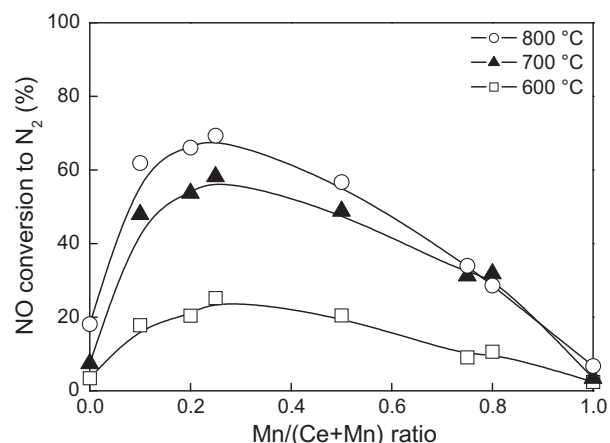
Fig. 1. Effect of the Mn/(Ce+Mn) ratio on NO conversion at various temperatures. Catalyst, 0.50 g; reaction gas, 6000 ppm NO in He; flow rate, 30 ml/min ( W/F = 1.0 \text{ g s ml}^{-1} ).
