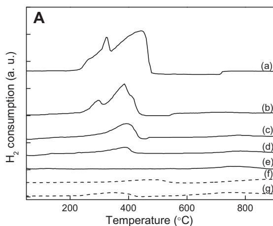
Fig. 5. H 2 -TPR profiles of Ce–Mn( x ) and BaO/Ce–Mn( x ) catalysts both calcined at 800 °C (except for A(f), (g) and B(a)). A: (a) Ce–Mn(1.0); (b) Ce–Mn(0.75); (c) Ce–Mn(0.5); (d) Ce–Mn(0.25); (e) Ce–Mn(0); (f) Ce–Mn(0) calcined at 600 °C and (g) Ce–Mn(0) calcined at 400 °C. B: (a) commercial Mn 2 O 3 as-received; (b) BaO/Ce–Mn(1.0); (c) BaO/Ce–Mn(0.75); (d) BaO/Ce–Mn(0.5); (e) BaO/Ce–Mn(0.25) and (f) BaO/Ce–Mn(0).
