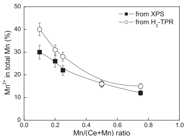
Fig. 7. Effect of Mn/(Ce+Mn) ratio on the Mn 2+ proportion in the Mn species calculated from the H 2 -TPR and XPS results of the BaO/Ce-Mn( x ) catalysts.
