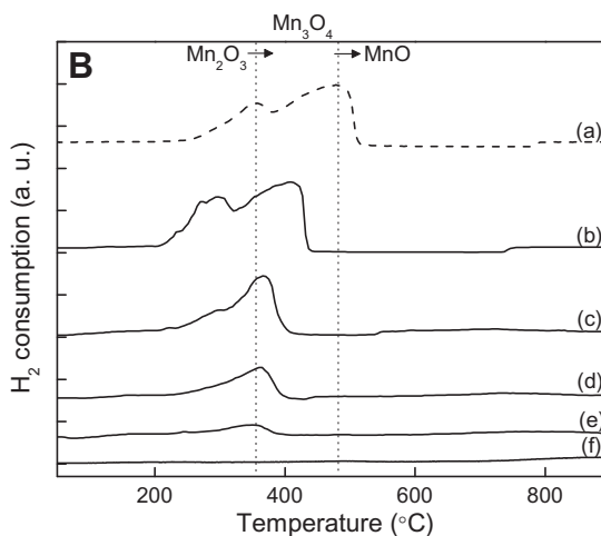
Fig. 5. H 2 -TPR profiles of Ce–Mn( x ) and BaO/Ce–Mn( x ) catalysts both calcined at 800 °C (except for A(f), (g) and B(a)). A: (a) Ce–Mn(1.0); (b) Ce–Mn(0.75); (c) Ce–Mn(0.5); (d) Ce–Mn(0.25); (e) Ce–Mn(0); (f) Ce–Mn(0) calcined at 600 °C and (g) Ce–Mn(0) calcined at 400 °C. B: (a) commercial Mn 2 O 3 as-received; (b) BaO/Ce–Mn(1.0); (c) BaO/Ce–Mn(0.75); (d) BaO/Ce–Mn(0.5); (e) BaO/Ce–Mn(0.25) and (f) BaO/Ce–Mn(0).
